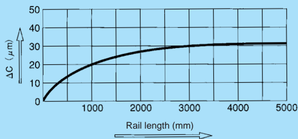
Fig. 7 Relationship Between LM-Rail Length and Running Parallelism
