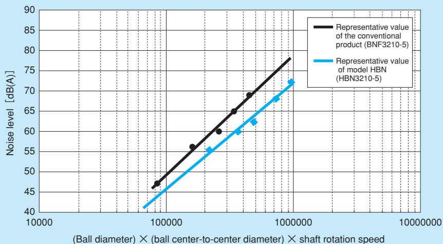
Fig. 5 Ball Screw Noise Level
